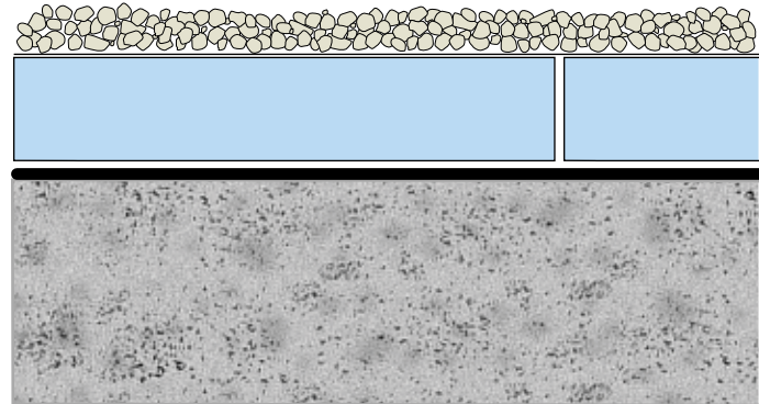
Protected Membrane Roof Assembly - membrane is protected
