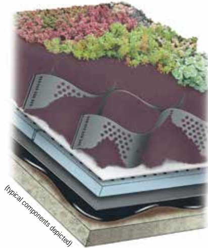
Sloped Garden Roof® Assembly
