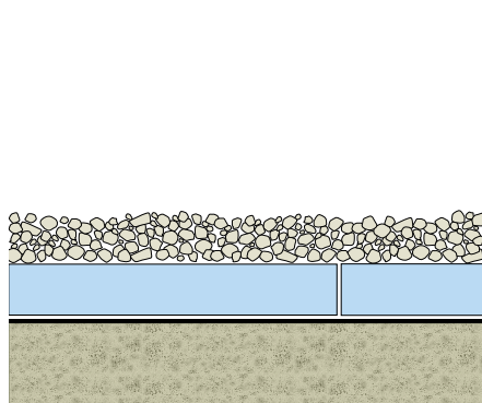
STYROFOAM ROOFMATE (40 psi)
