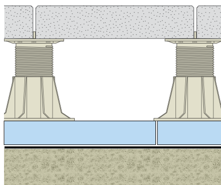
STYROFOAM PLAZAMATE (60 psi)
