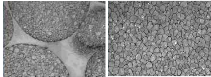
EPS - Open Cell (mag. 25x)
