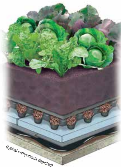
Urban Agriculture Garden Roof® Assembly
