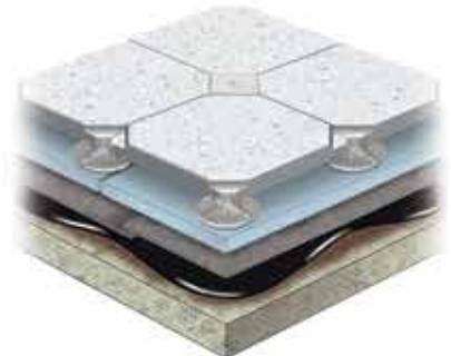
Ultimate Assembly Guardian Pavers
